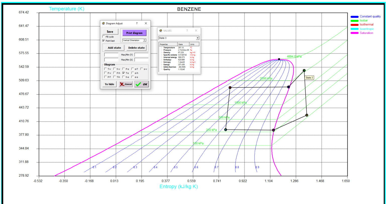
Graphic representations of a thermodynamic cycle
