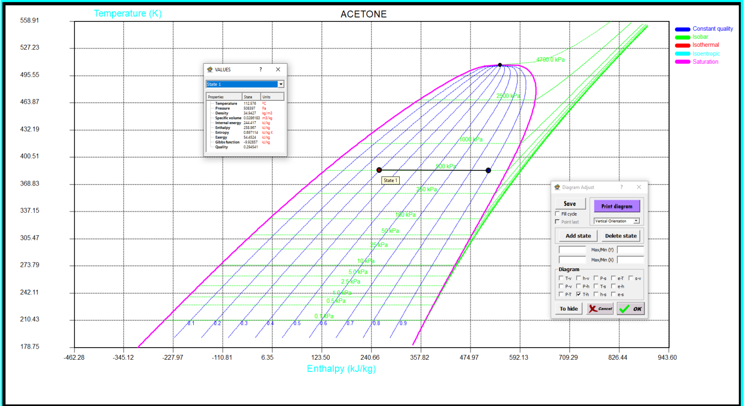
Graphic representations of a thermodynamic process
